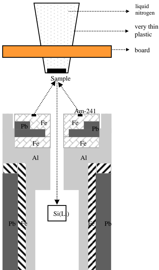
Figure1. Experimental setup
